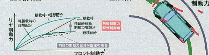
●EBD(電子制動力配分制御) = Electronic Brake force Distribution
